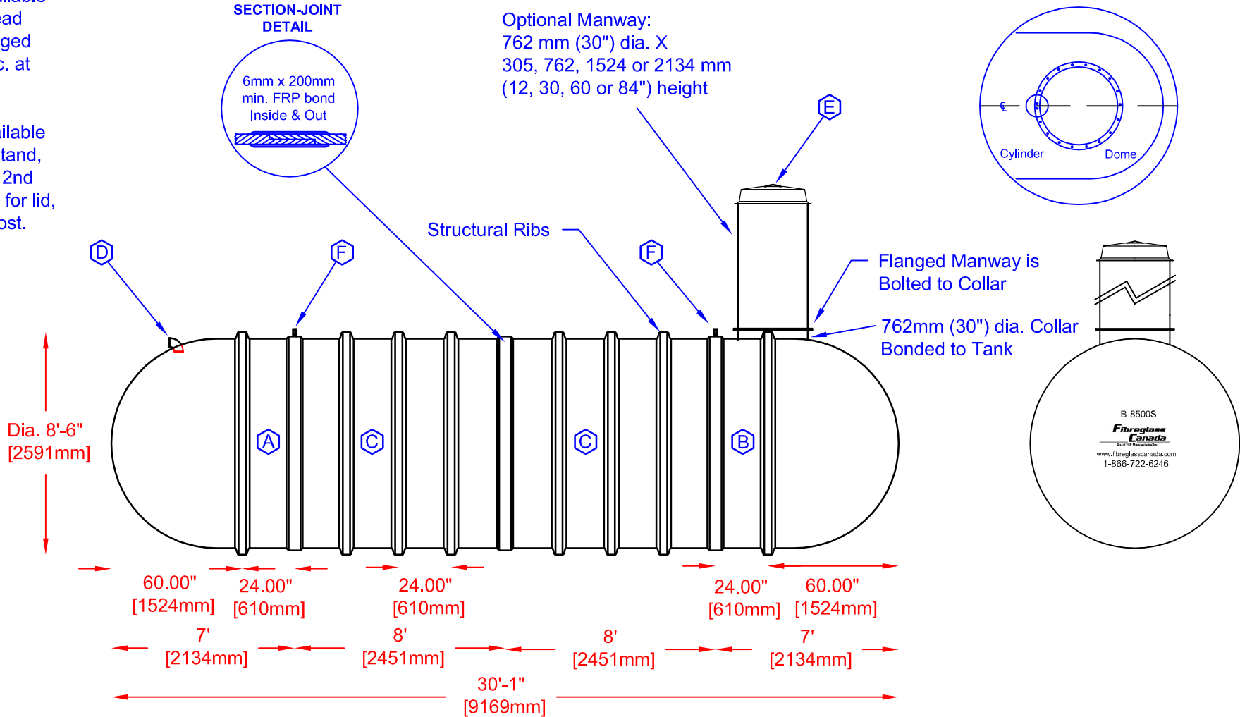
COLLAR ORIENTATION DETAIL
