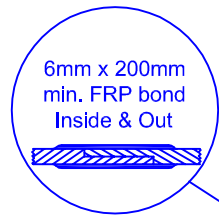
SECTION-JOINT DETAIL
