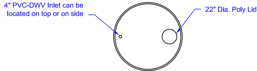
TOP VIEW
