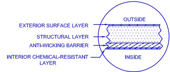
LAMINATE DETAIL
