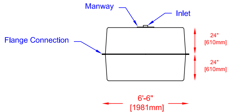
END VIEW
