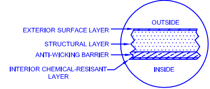
LAMINATE DETAIL
