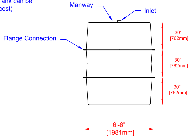
END VIEW
