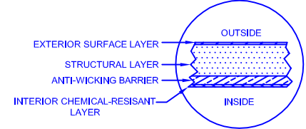
LAMINATE DETAIL
