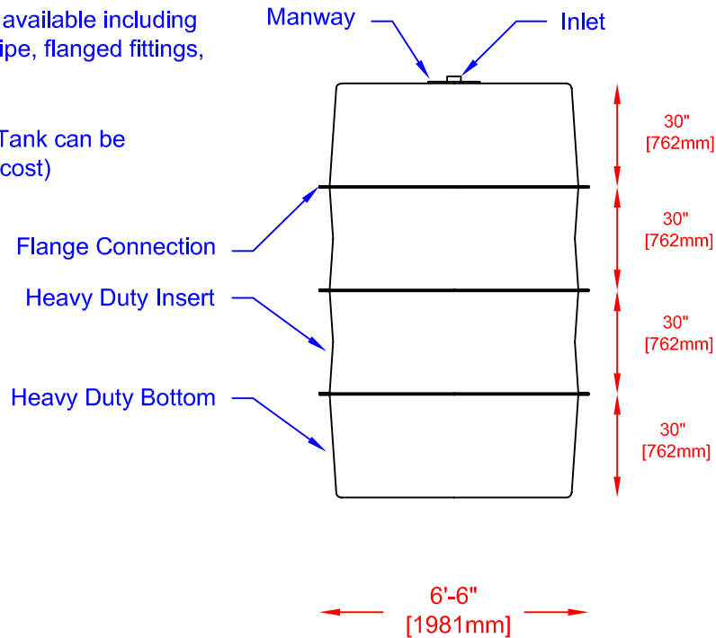
END VIEW
