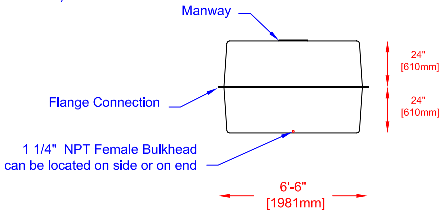
END VIEW
