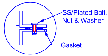
FLANGE CONNECTION DETAIL
