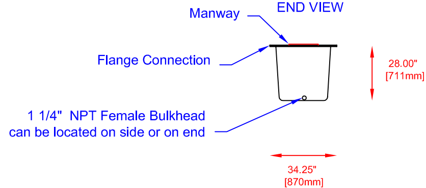
END VIEW
