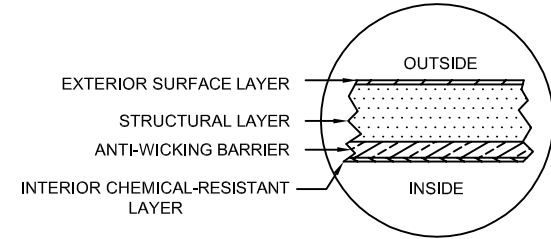
LAMINATE DETAIL
