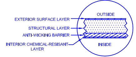
LAMINATE DETAIL
