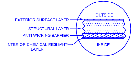
LAMINATE DETAIL
