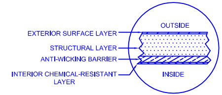
LAMINATE DETAIL
