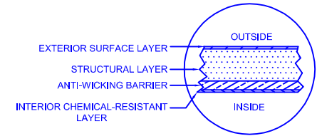
LAMINATE DETAIL
